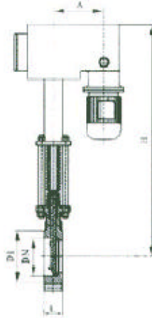
主要外型及连接尺寸 Main External And Connecting Dimensions(mm)
